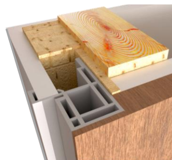
Out-swing Profile
